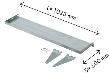
10360042385 Kulmahylly S600mm
